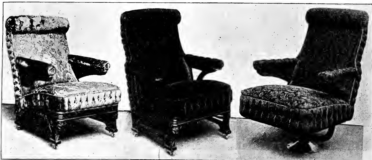
Figs. 3977-3979. SCARRITT'S DRAWING-ROOM-CAR CHAIRS.
